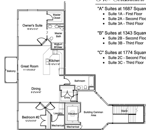
Suite 2B and 3B Floor Plan
