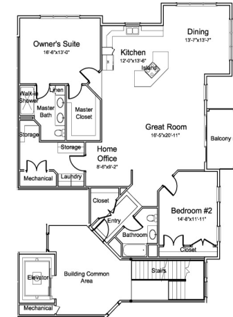
Suite 2A and 3A Floor Plan
