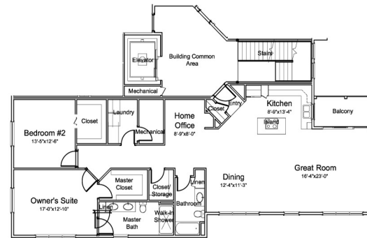
Suite 2C and 3C Floor Plan
